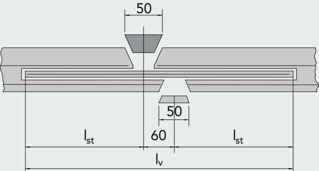
FIG. 15 EMPALME DE DOS LONAS CON LONA INTERMEDIA SPLICING TWO PLYS WITH PLY IN THE MIDDLE
