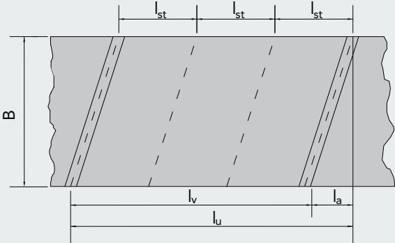
FIG. 16 ESQUEMA GENERAL DE EMPALME ESCALONADO GENERAL VIEW OF STEPPED SPLICE
